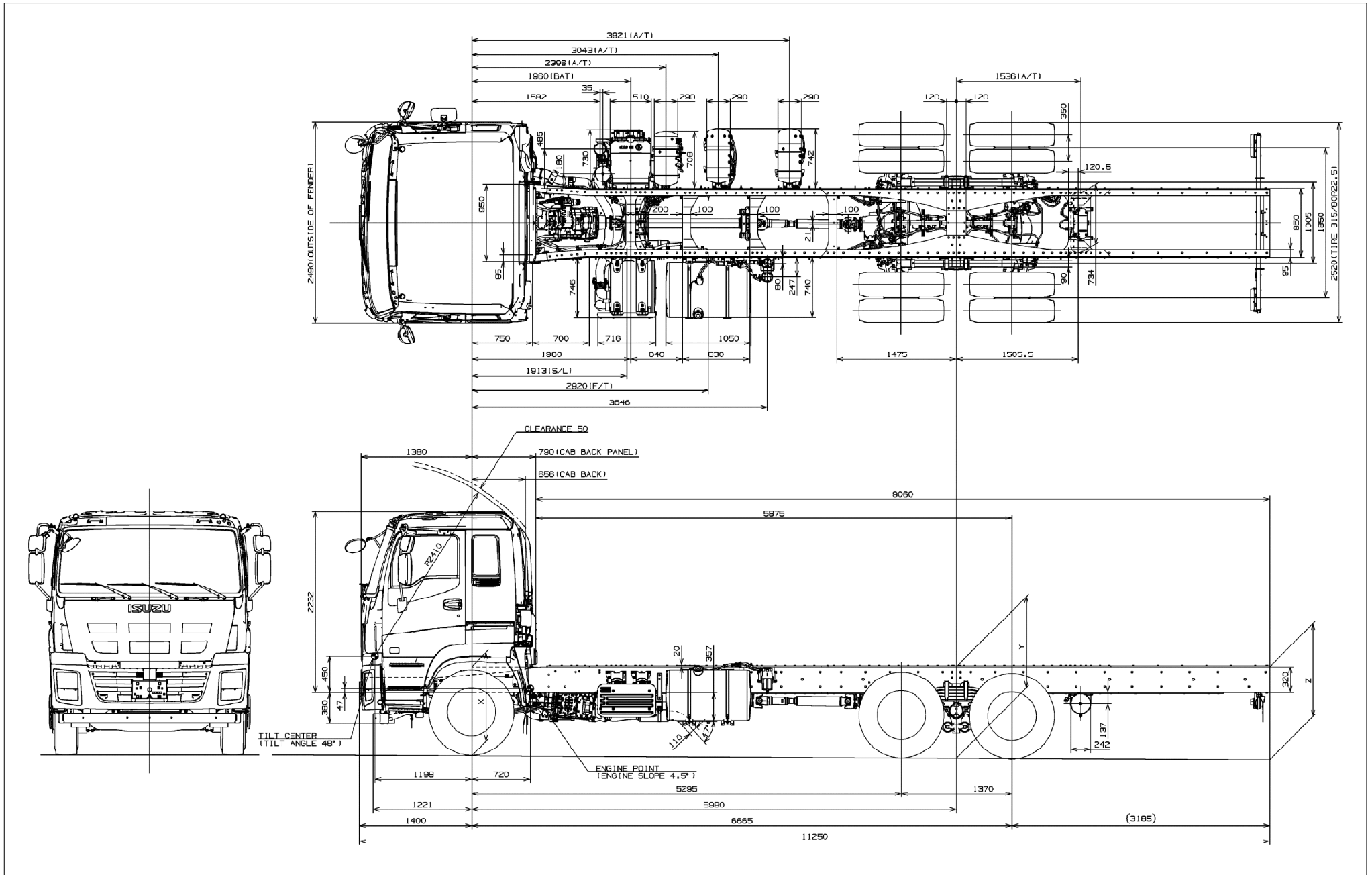
Fig. 9-1-7 Cab Chassis Drawing CYZ52TLC3T17
